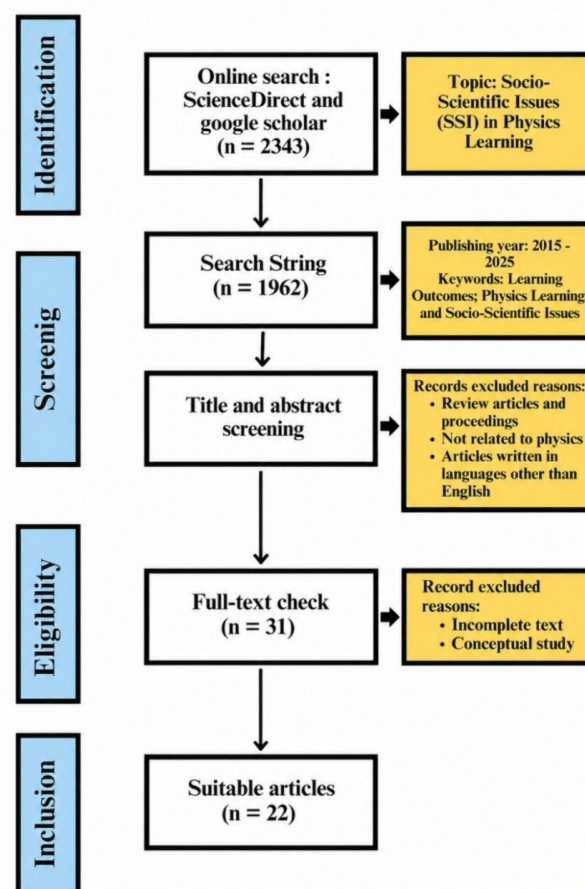
Figure 1. PRISMA flow diagram of article selection process
